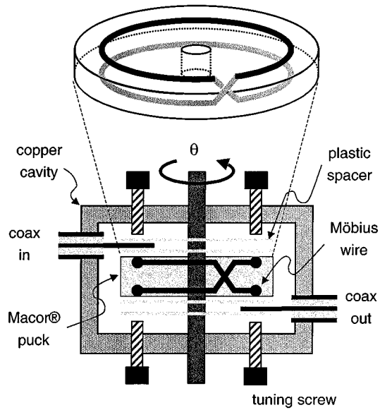
Fig. 7. (top) Perspective drawing of the dielectric-loaded Möbius wire resonator showing the Macor puck and the embedded gold wire with the cross over accomplished with two vias. (bottom) Edge view of a two-pole filter consisting of a dual-mode dielectric-loaded Möbius wire resonator in a copper cavity.
