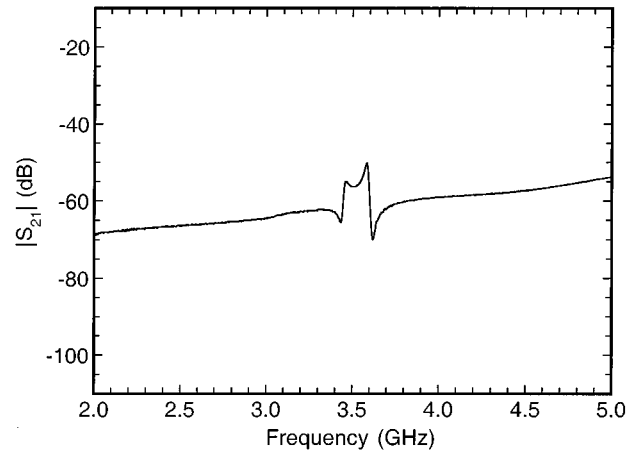
Fig. 9. Weakly coupled response of the dielectric-loaded Möbius wire resonator shown in Fig. 7.
