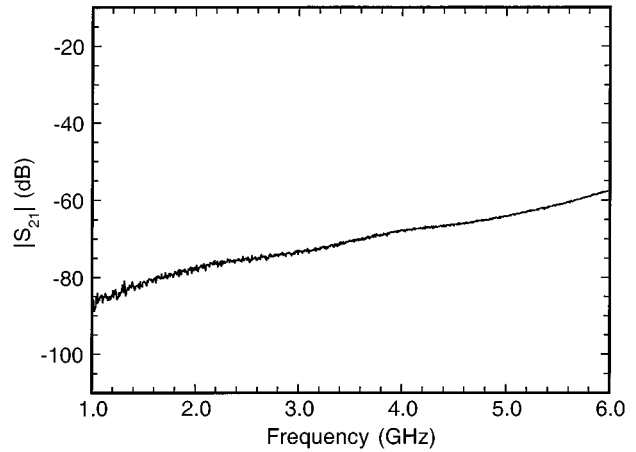
Fig. 8. The 1.0–6.0-GHz response of a “control” Macor cylinder without an embedded Möbius wire resonator.
