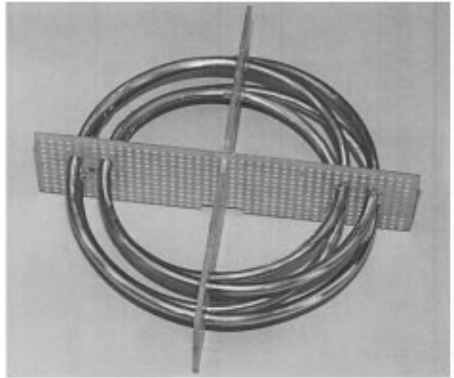
Fig. 4. Photograph of the quad-mode Möbius wire resonator that is placed in an 11.43-cm-diameter 3.175-cm-high cylindrical aluminum cavity.
