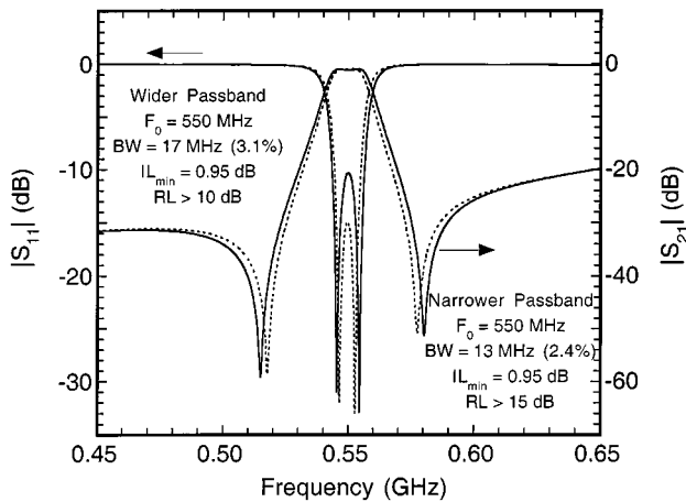
Fig. 2. Measured responses of the two-pole two-zero bandpass filter, consisting of a dual-mode Möbius resonator, when tuned for two different bandwidths.
