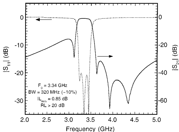
Fig. 12. Tuned four-pole four-zero bandpass filter response of the dielectric-loaded Möbius wire resonator filter shown in Fig. 11.
