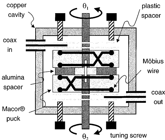
Fig. 11. Edge view of a four-pole filter consisting of two cascaded dual-mode dielectric-loaded Möbius wire resonators in a copper cavity.
