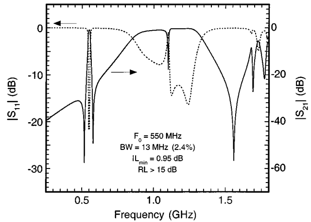
Fig. 3. Measured out-of-band response of the two-pole bandpass filter, consisting of a dual-mode Möbius resonator, when tuned for the narrower bandwidth.
