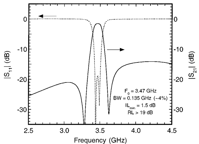
Fig. 10. Tuned two-pole two-zero bandpass filter response of the dielectric-loaded Möbius wire resonator filter shown in Fig. 7.
