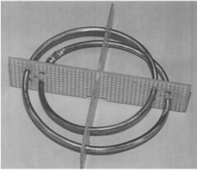
Fig. 1. Photograph of the dual-mode Möbius wire resonator that was placed in an 11.43-cm-diameter 3.175-cm-high cylindrical aluminum cavity.
