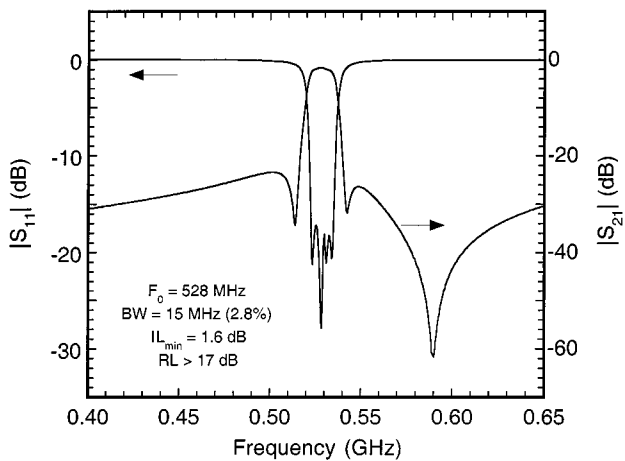
Fig. 6. Response of the four-pole bandpass filter, consisting of a single quad-mode Möbius resonator, tuned for best passband response.
